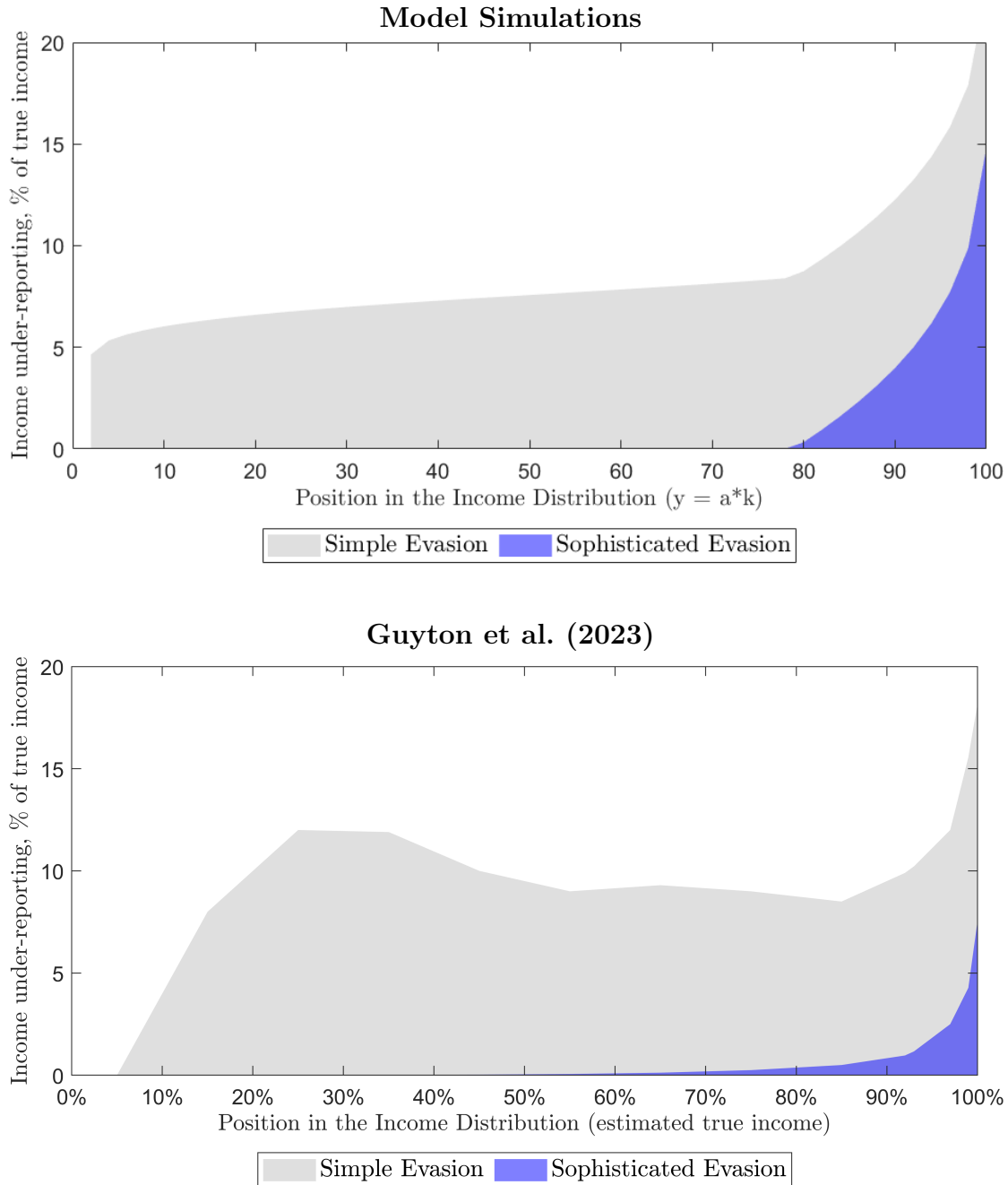
Figure 7: Comparison of Model Simulations and Estimates on US Unreported Income, by Percentile of Income (as % of True Income y_t ), Average 2006-2013. The top panel shows the model estimates of unreported income, while the bottom panel presents the corresponding real data as estimated by Guyton et al. (2023). Both plots display the distribution of simple and sophisticated evasion across percentiles of income.
