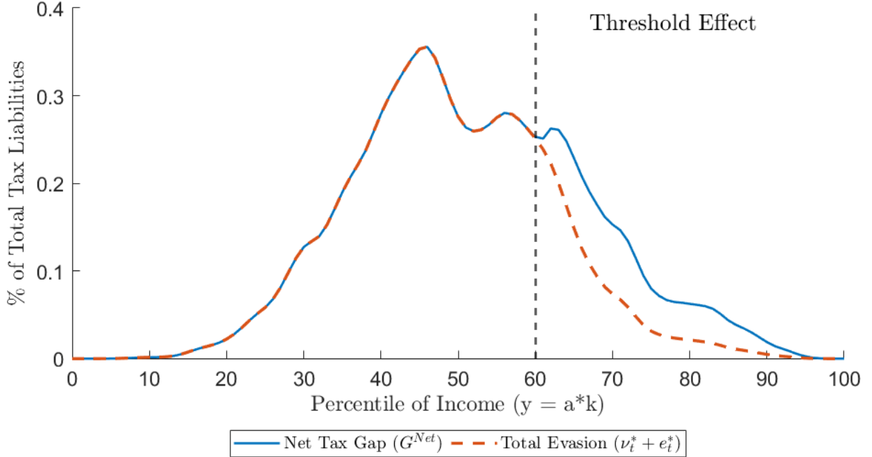
Figure 6: Distribution of Net Tax Gap and Evasion Contributions This figure depicts the amount of evasion and net tax gap contributed to the total amounts by income group, weighted by the amount of wealth held by agents across the distribution.
