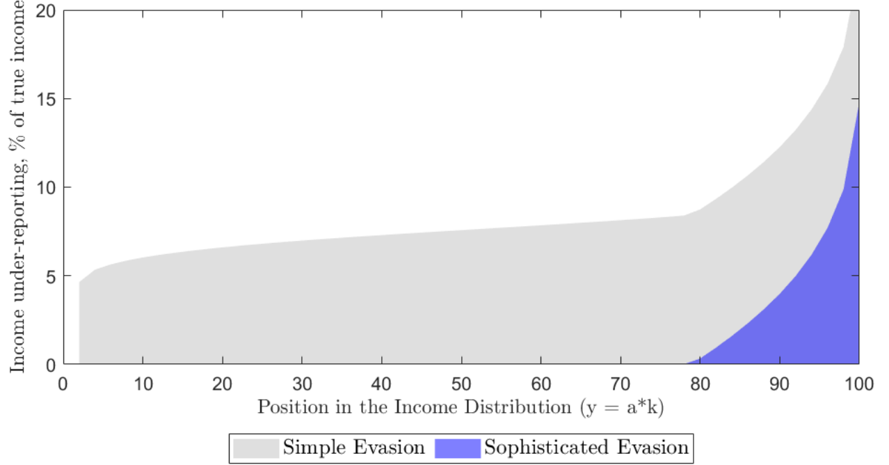
Figure 2: Model Estimates of U.S. Unreported Income by Percentile of Income, Average 2006-13 (as % of True Income y_t ) . This figure plots the models simulated estimates of tax payers' optimal under-reported income by evasion strategy, optimal evasion type ( e_t^*, \nu_t^* ) and over their position in the simulated stationary income distribution.
